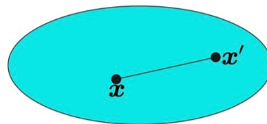
Convex
